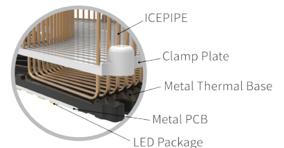
Heat sink
